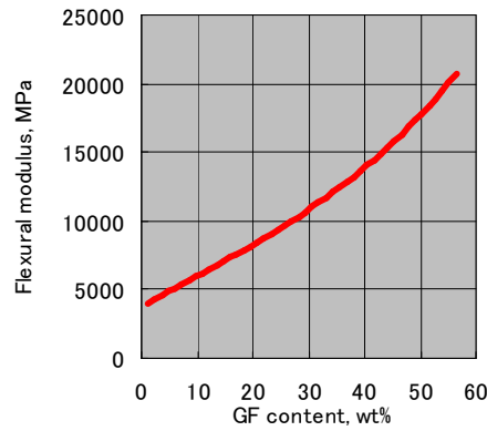
Fig.3 Flexural modulus
