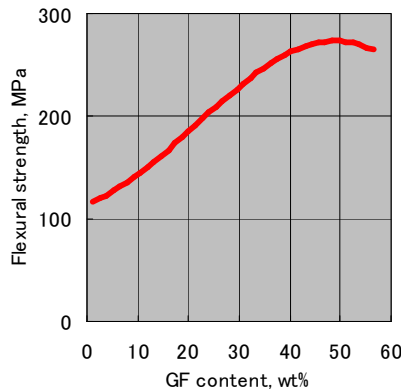
Fig.2 Flexural strength
